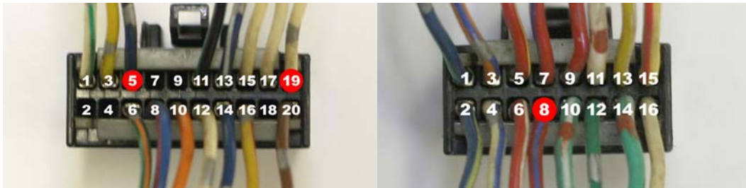
B - Plug
