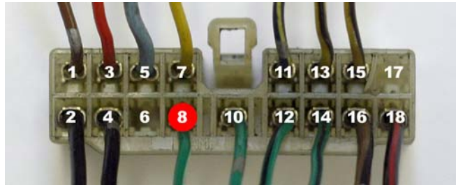
A - Plug
